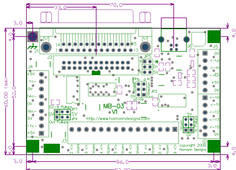
Illustration 1: MB-03 Layout
