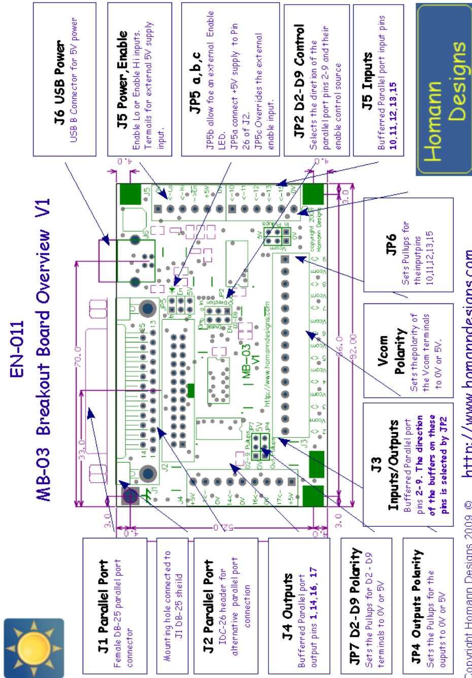
Illustration 3: MB-03 Breakout Board Overview
